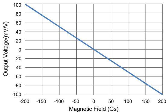
Figure 2. TMR2584 output curve
