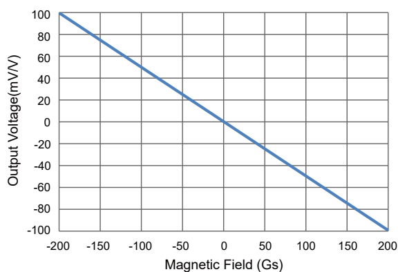
TMR2584 ±200 Gs Output Curve
